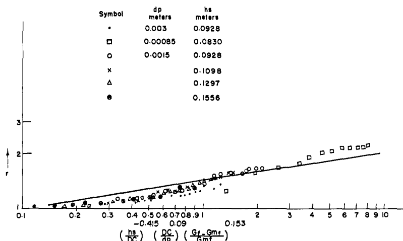
Fig. 3. Variation of r with system parameters
