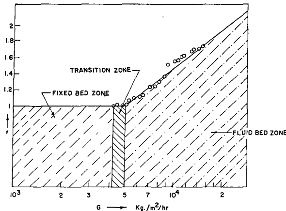
Fig. 2. Variation of r with fluid mass velocity.
