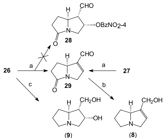
Scheme 9. (a) O_3 , CH_2Cl_2 , -78\text{ }^\circ\text{C} , then Ph_3P , 50%; (b) Red-Al, THF, reflux (3 h), 76% (c) O_3 , CH_2Cl_2 , -78\text{ }^\circ\text{C} ; then excess Red-Al, THF, reflux (3 h), 33%.
