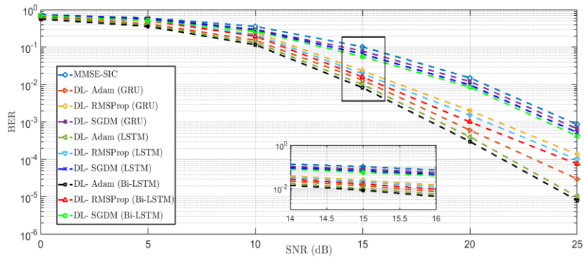
Figure 7. BER performance with cyclic prefix 16 for User 1
