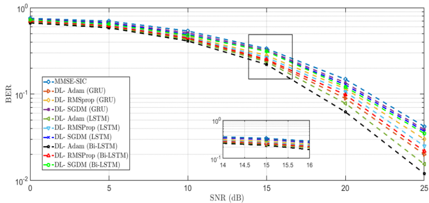
Figure 8. BER performance with cyclic prefix 16 for User 2
