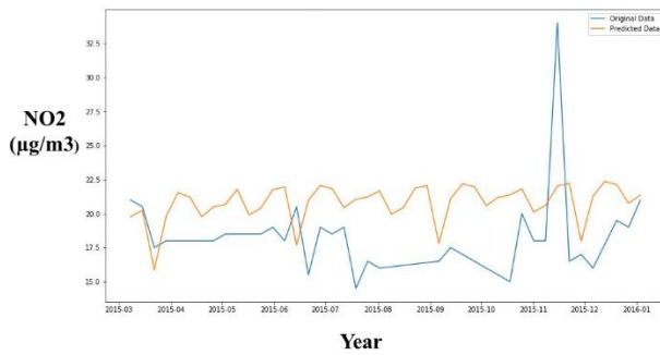
Figure 8. SARIMA model-NO2
