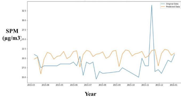
Figure 7. SARIMA model-SPM
