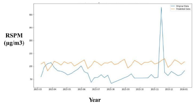
Figure 10. SARIMA model-RSPM
