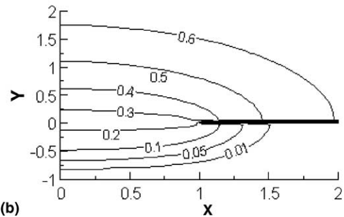
Fig. 6. Etched profiles and concentration distribution for \beta = 10 and infinitely thin mask: (a) comparison of etched profiles with the variational inequality approach, (b) concentration contour at t^* = 20 .
