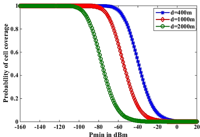
Fig 4 Coverage probability vs P_{min}
