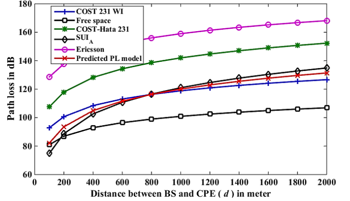
Fig 3 Comparison of predicted PL model with standardised PL models
