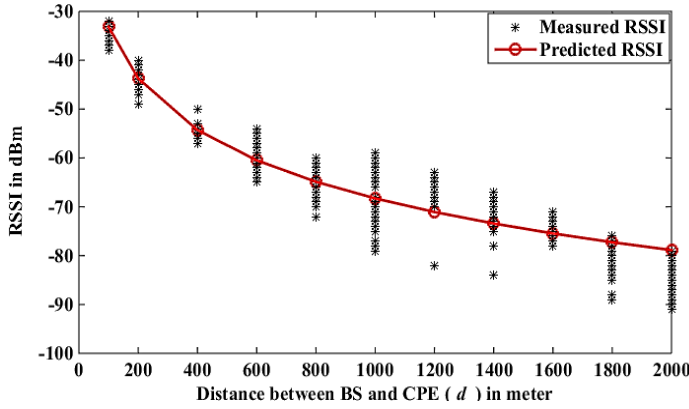
Fig 2 Predicted RSSI model
