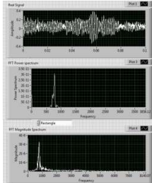
Fig. 7: FFT of recorded signal for GFRE composite
