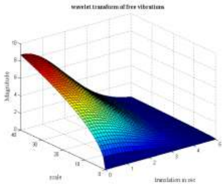
Fig. 4: Morlet Wavelet Transform of boring bar vibrations composite
