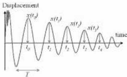
Fig. 3: Logarithmic decrement plot
