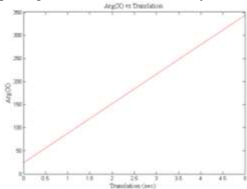
Fig. 6: Phase vs translation plot for GFRE composite
