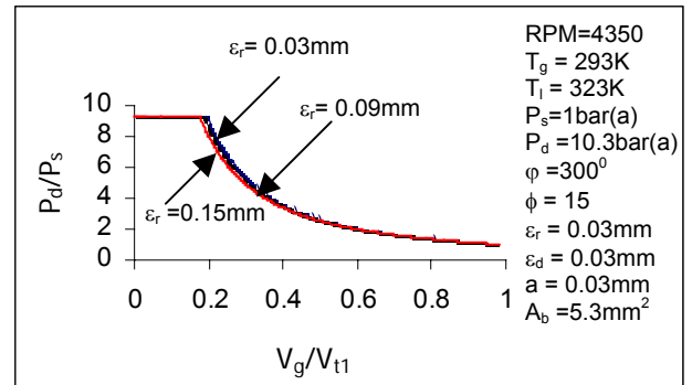
Figure 4 Effect of interlobe clearance on P- V diagram profile
