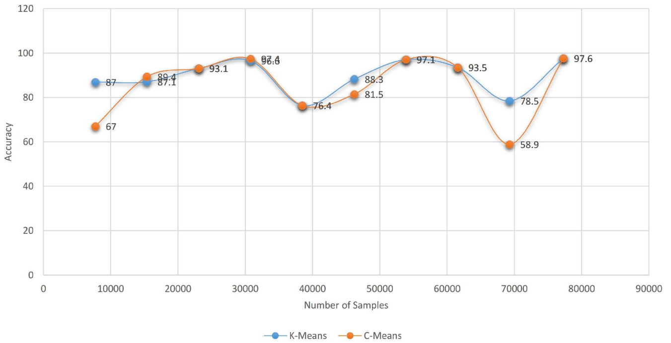
Fig. 9. Comparison of K-Means and C-Means on KDD Corrected Dataset
