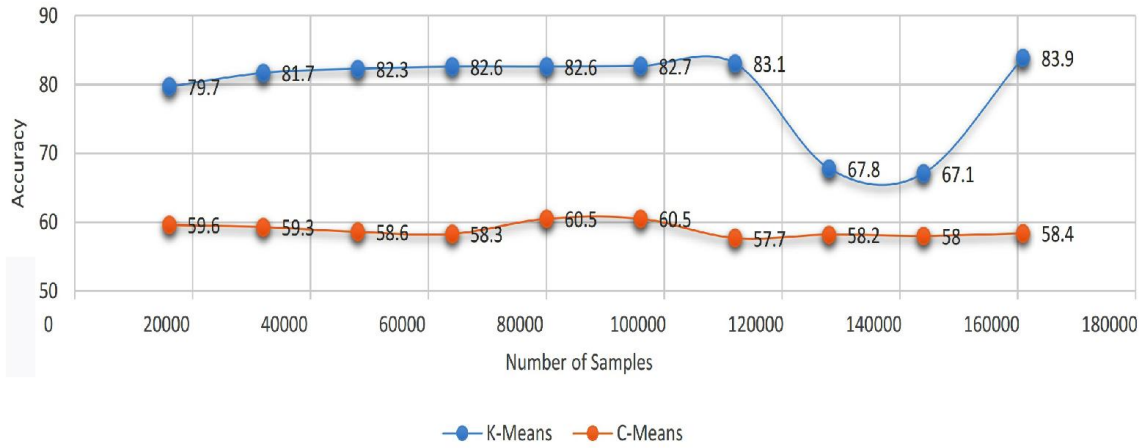
Fig. 12. Comparison of K-Means and C-Means on GureKDD dataset.
