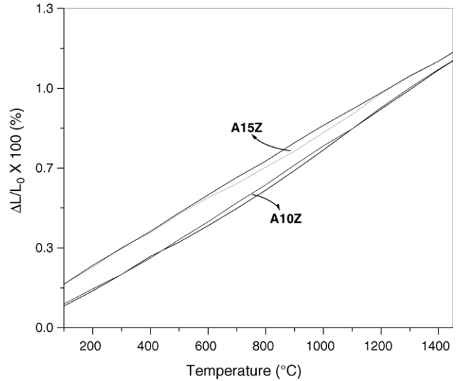
Fig. 10. Thermal expansion curve of Al 2 O 3-x ZrO 2 (where x = 10 and 15 mol.%) sintered at 1550 °C/4 h.
