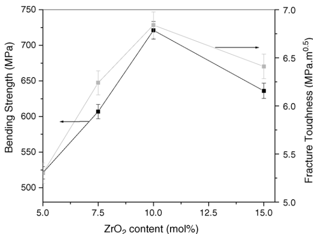
Fig. 8. Bending strength and fracture toughness of ZTA composite as a function of ZrO 2 .
