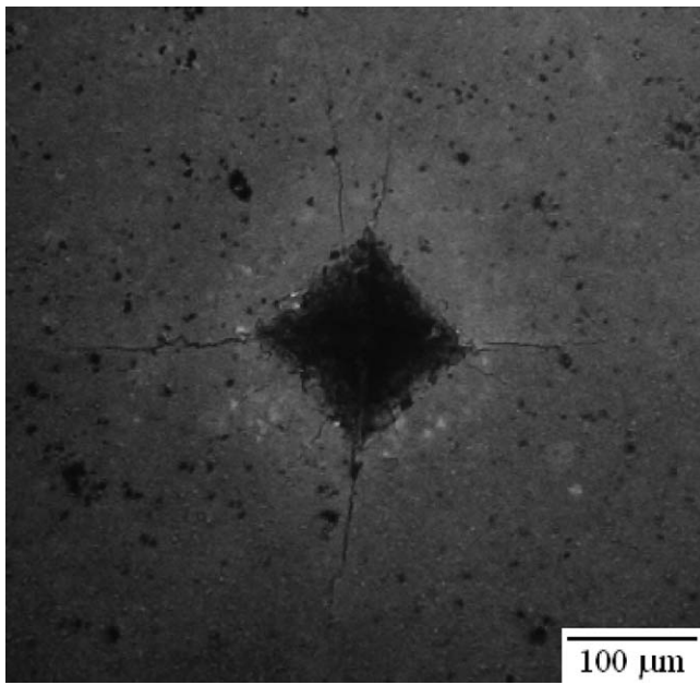
Fig. 7. The Vickers indentation (at 5 kg indent load) on the A10Z ceramic and the propagation of the radial cracks.
