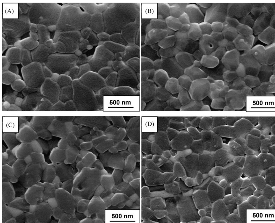
Fig. 4. SEM microstructure of fracture surface of \text{Al}_2\text{O}_3\text{-ZrO}_2 composite sintered at 1550\text{ }^\circ\text{C} for 4 h, represented as A5Z (A), A7.5Z (B), A10Z (C), A15Z (D). The phases with gray and white contrast indicate \text{Al}_2\text{O}_3 and \text{ZrO}_2 , respectively. The black irregular shape represents the corresponding pores in the sintered body.
