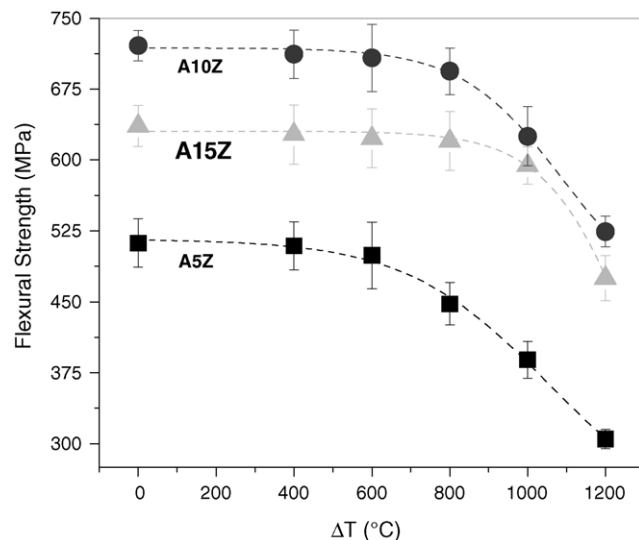
Fig. 9. Plot of retained flexural strength vs. thermal shock temperature for Al 2 O 3 with variation of ZrO 2 .
