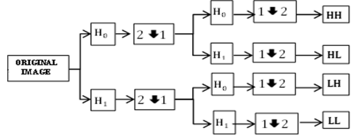
Fig.5 Discrete wavelet decomposition with filter banks
