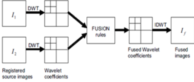
Fig.7 DWT based Image Fusion Flow chart
