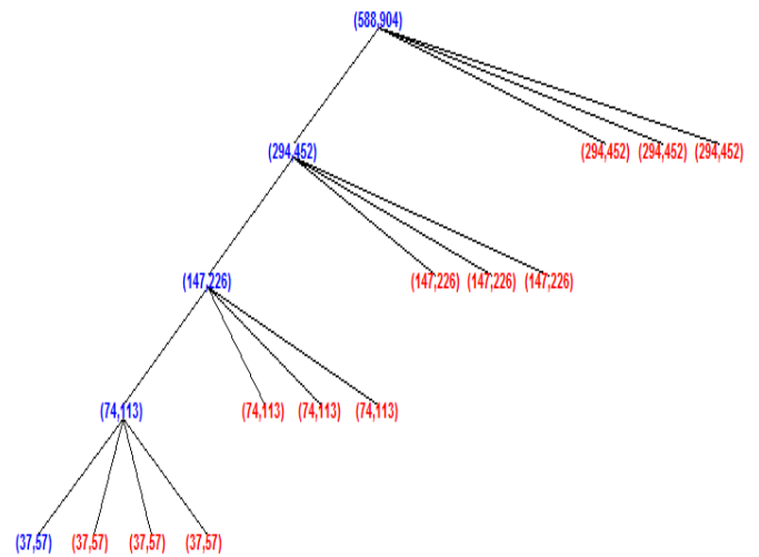
Fig.12 Haar Wavelet decomposition tree at 4 th level
