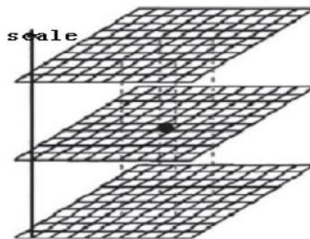
Fig. 2 Local extremum in DoG scale space
