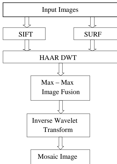
Fig.1 Flow chart for proposed technique
