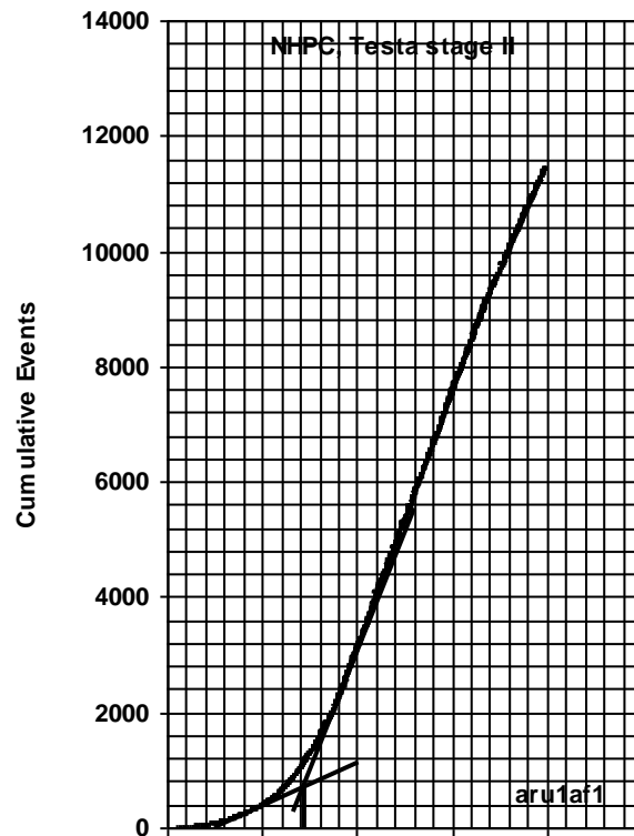
Figure 4. AE parameter plots for site-1
