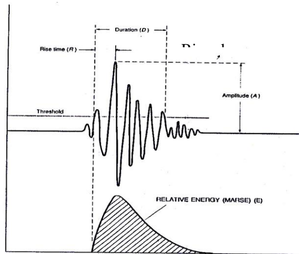
Figure 3. Acoustic emission wave form parameters ( Pollock, 1980)
