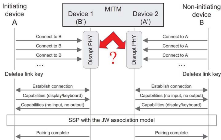
Fig. 2. MITM Attack on Bluetooth SSP
