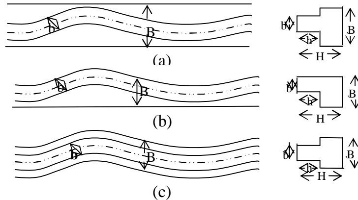
FIG. 1(b) Plan Forms of Meandering Experimental Channels with Floodplains
