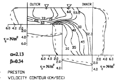
Fig. 2(b) Isovel and Boundary shear stress distribution Of Meandering Channel with one side Flood plain
