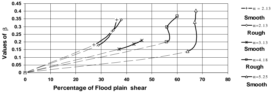
FIG. 4 Variation % of Flood plain shear with relative depth
