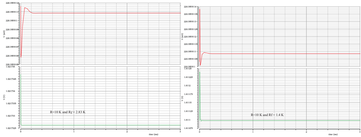
(a) Output of LDO V_{ref} = 1 V.
