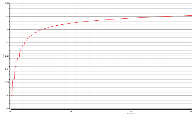
(c) Output of LDO V_{ref} = 3.3 V.
