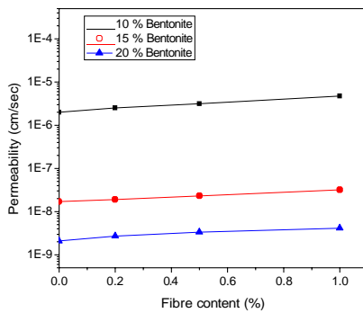
Fig. 10. Variation of hydraulic conductivity with fibre content
