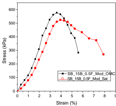
Fig. 8. Effect of water content on stress-strain curve
