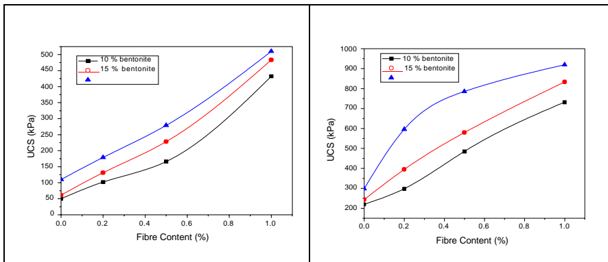
Fig. 4. Effect of addition of fibre for lightly compacted sample at their OMC
