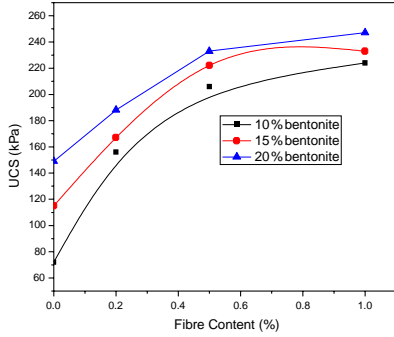
Fig. 6. Effect of addition of fibre for lightly compacted sample at saturated condition
