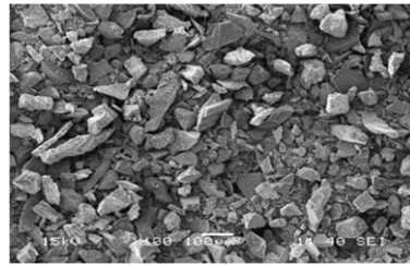
Fig. 2. Microscopic angular structure of sand by SEM
