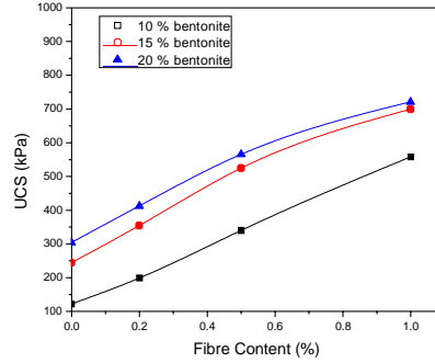
Fig. 7. Effect of addition of fibre for heavily compacted sample at saturated condition
