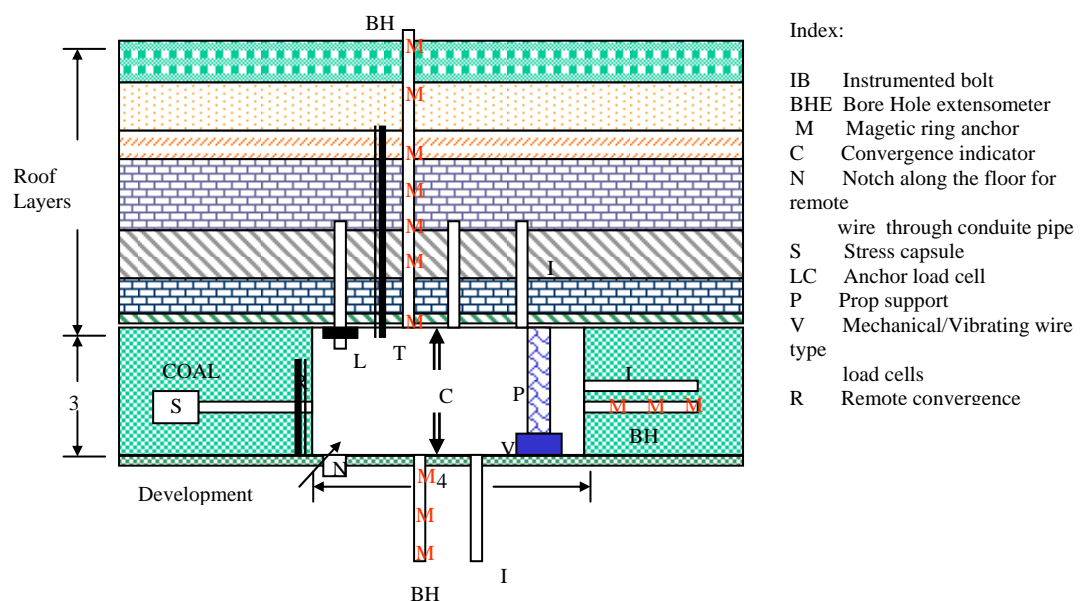
Fig 1: Typical instrumentation for strata monitoring around underground workings.
