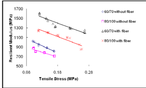
Fig. 2 Variation of Resilient moduli with Tensile stress at different temperatures
