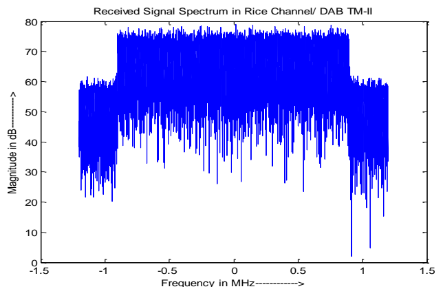
Figure 9. Received signal spectrum in Rician channel.
