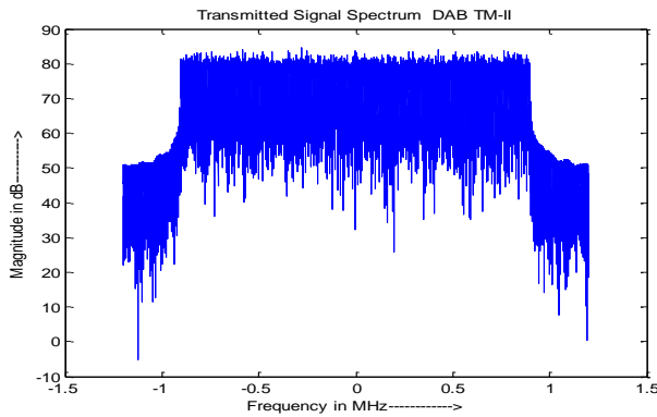
Figure 6. Transmitted signal spectrum.
