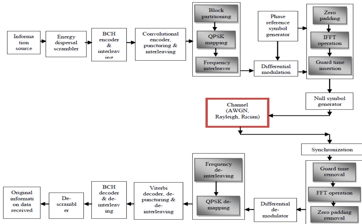
Figure 3. Block diagram of system simulated.
