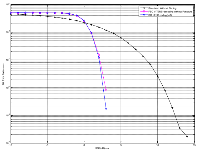
Figure 13. BER performance with concatenated coding in Rician channel.
