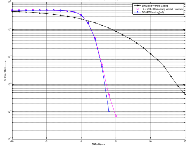
Figure 12. BER performance with concatenated coding in Rayleigh fading channel.
