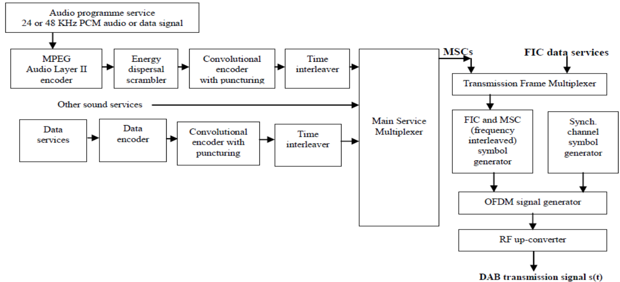
Figure 1. Complete DAB transmitter block diagram [1].
