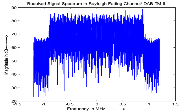
Figure 8. Received signal spectrum in Rayleigh fading channel.
