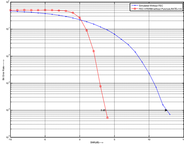
Figure 10. BER performance with and without FEC coding in AWGN channel.
